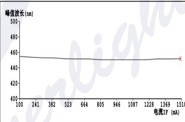
Spectral wavelength
